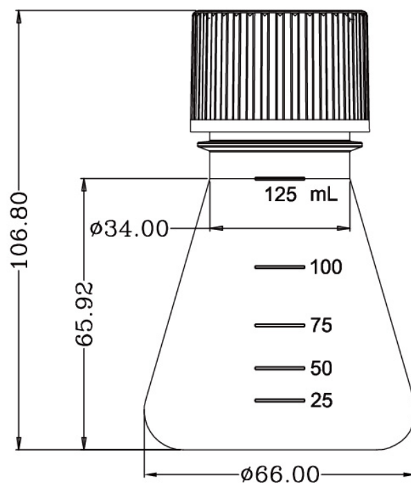
125mL Erlenmeyer Flask
